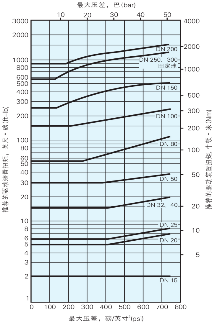
PTFE(T)密封座阀门
