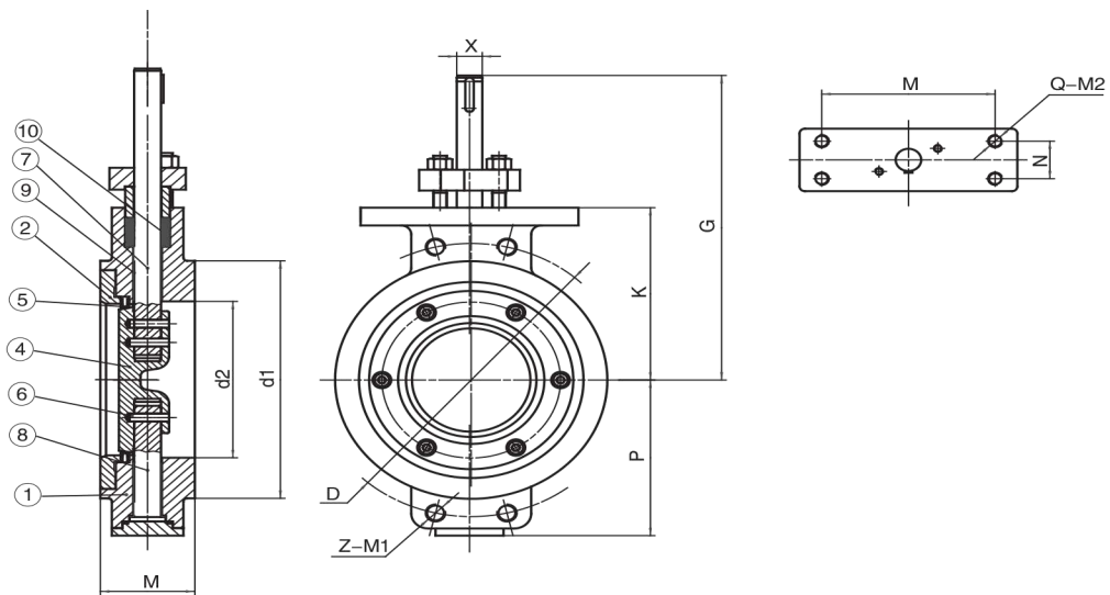
HP8-150W 饼式蝶阀尺寸 CLASS 150
